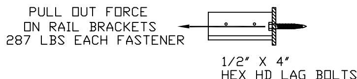
RAIL REACTIONS
